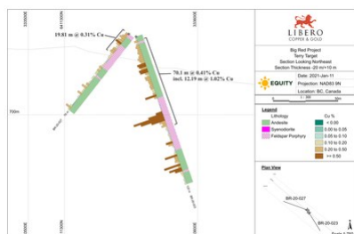
Figure 1: Cross-section of drill holes BR-20-23 and BR-20-27 (CNW Group/Libero Copper & Gold Corporation.)
